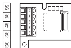
FX1N-4EX-BD
