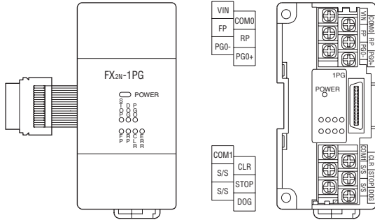
FX2N-1PG-E
