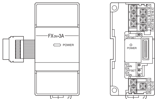
FX0N-3A V IN 2 I IN 2 COM2 V IN 1 I IN 1 COM1 V OUT I OUT COM
