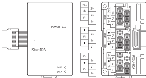
FX3U-4DA
