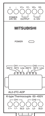
AL2-2TC-ADP
