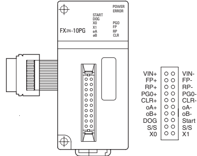
FX2N-10PG
