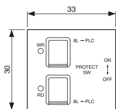
FX1N-EEPROM-8L
