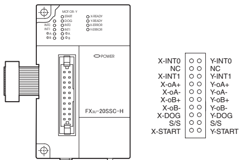
FX3U-20SSC-H
