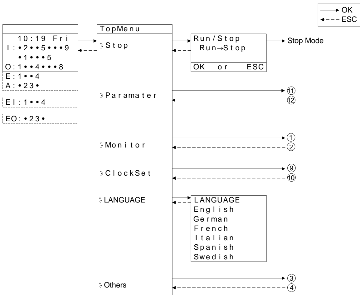
Figure 3.8: TopMenu in Run Mode Operation
