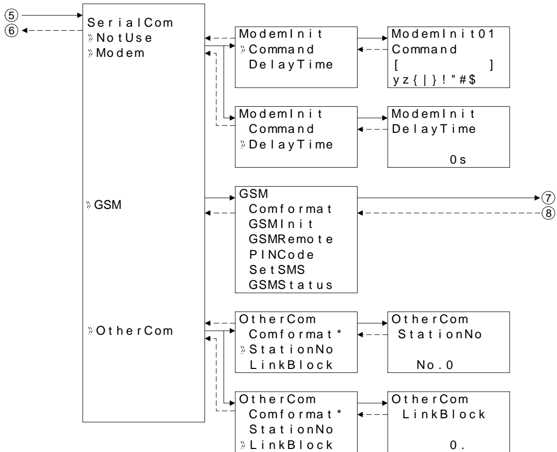
Figure 3.10: Serial Com in Run Mode operation (AL2-14MR-*, AL2-24MR-*)
