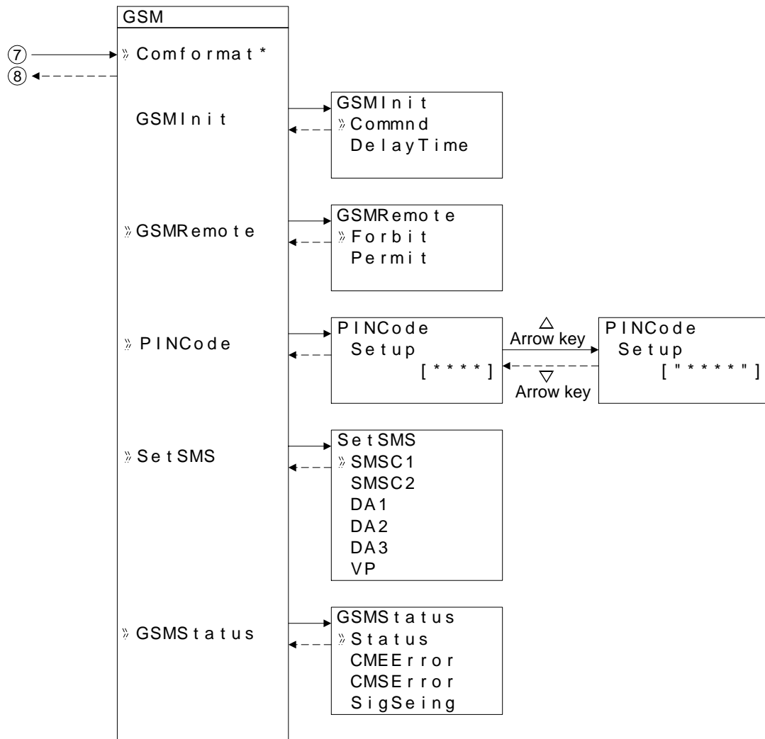
Figure 3.5: GSM Menu in Stop Mode operation
