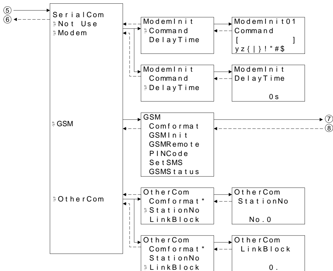
Figure 3.3: Serial Com in Stop Mode operation (AL2-14MR-*, AL2-24MR-*)
