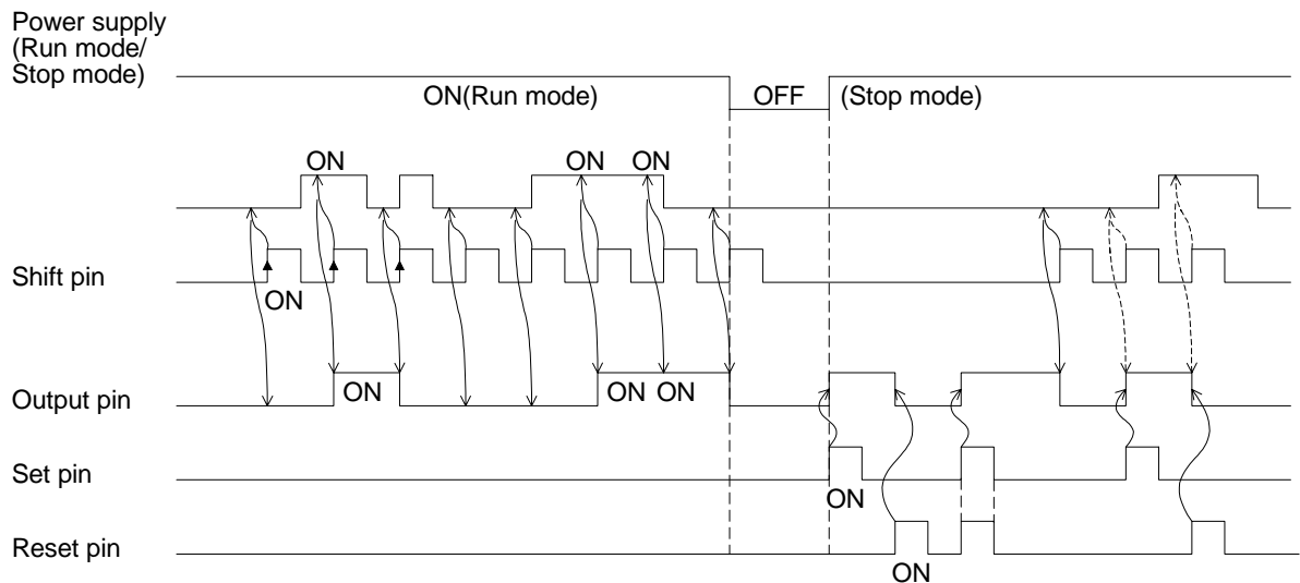
1) Shift Operation Timing Diagram
