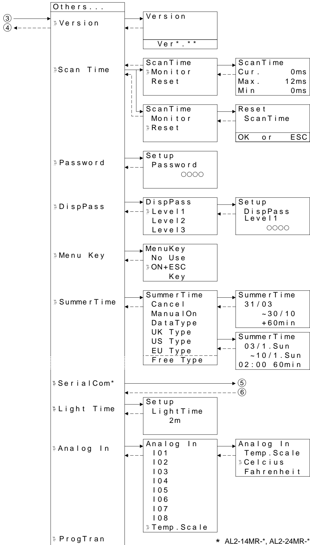
Figure 3.9: Others Menu in Run Mode operation
