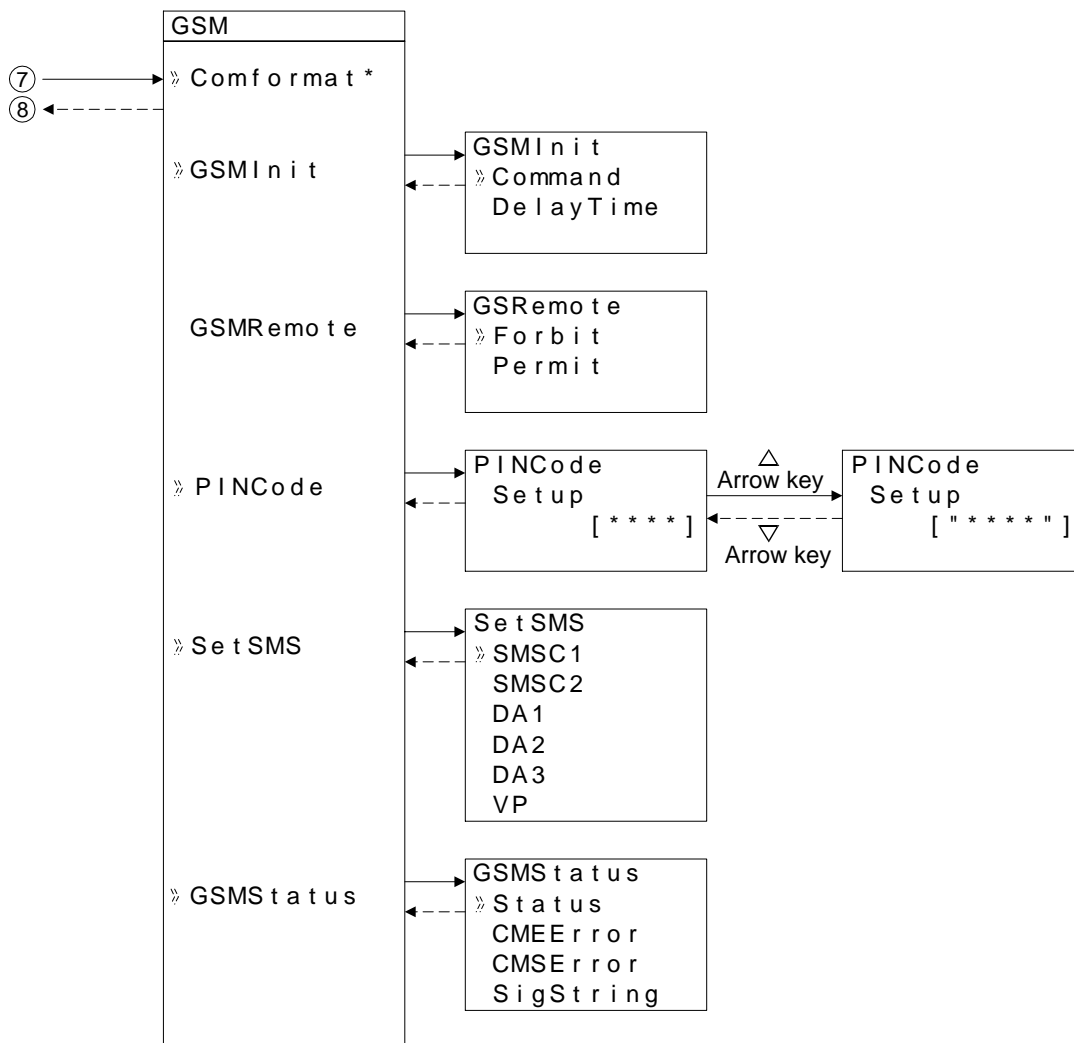
Figure 3.12: GSM Menu in Run Mode operation (AL2-14MR-*, AL2-24MR-*)
