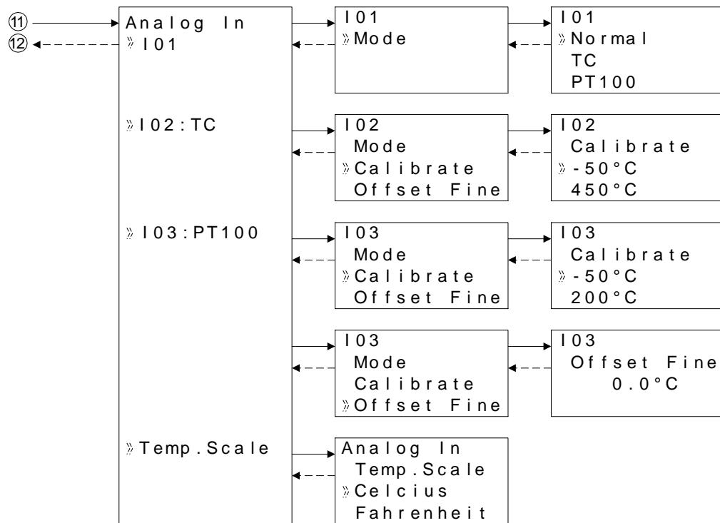
Figure *.*: Analog Inputs Setup Menu.
