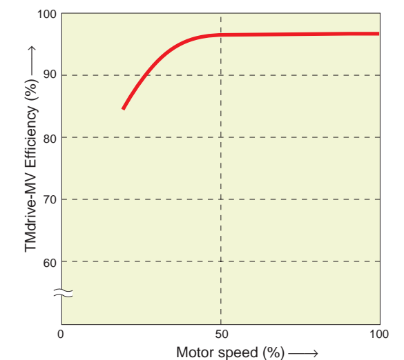
● Expected input power factor of TMdrive-MV
